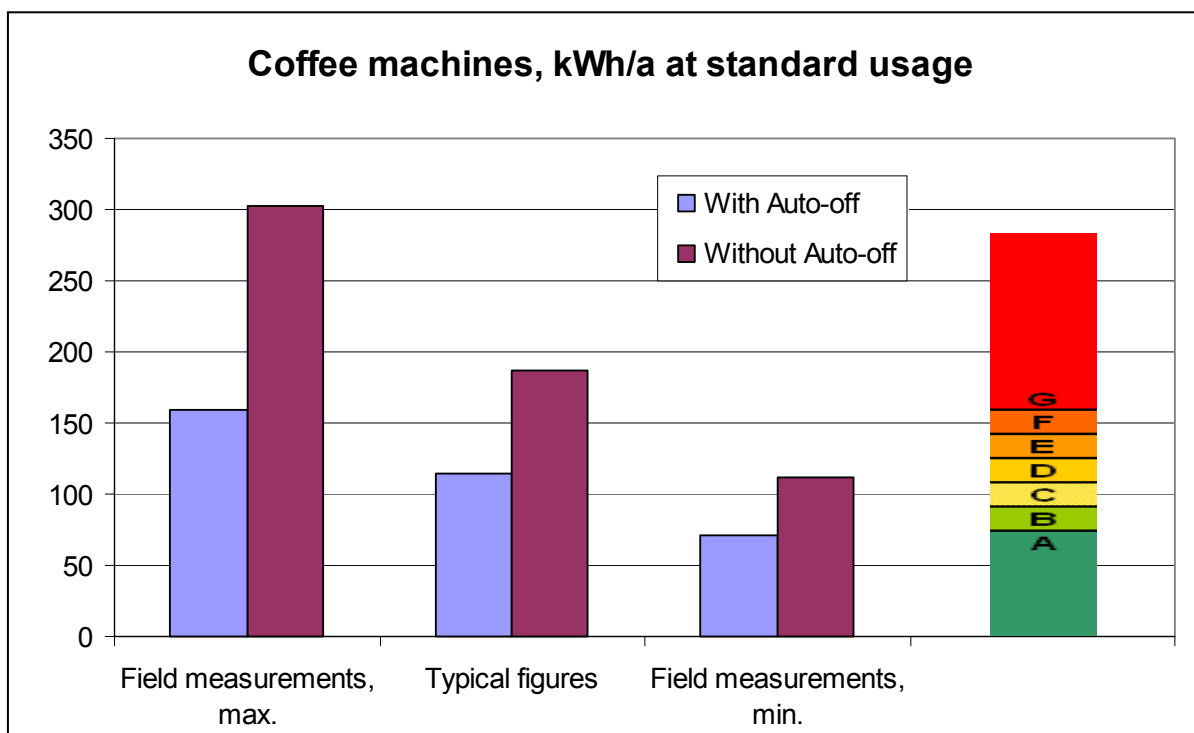
Fig. 2 Energy consumption of coffee machines at standard usage and possible energy label scheme
